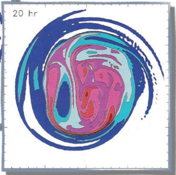
PV mixing in Hurricanes
